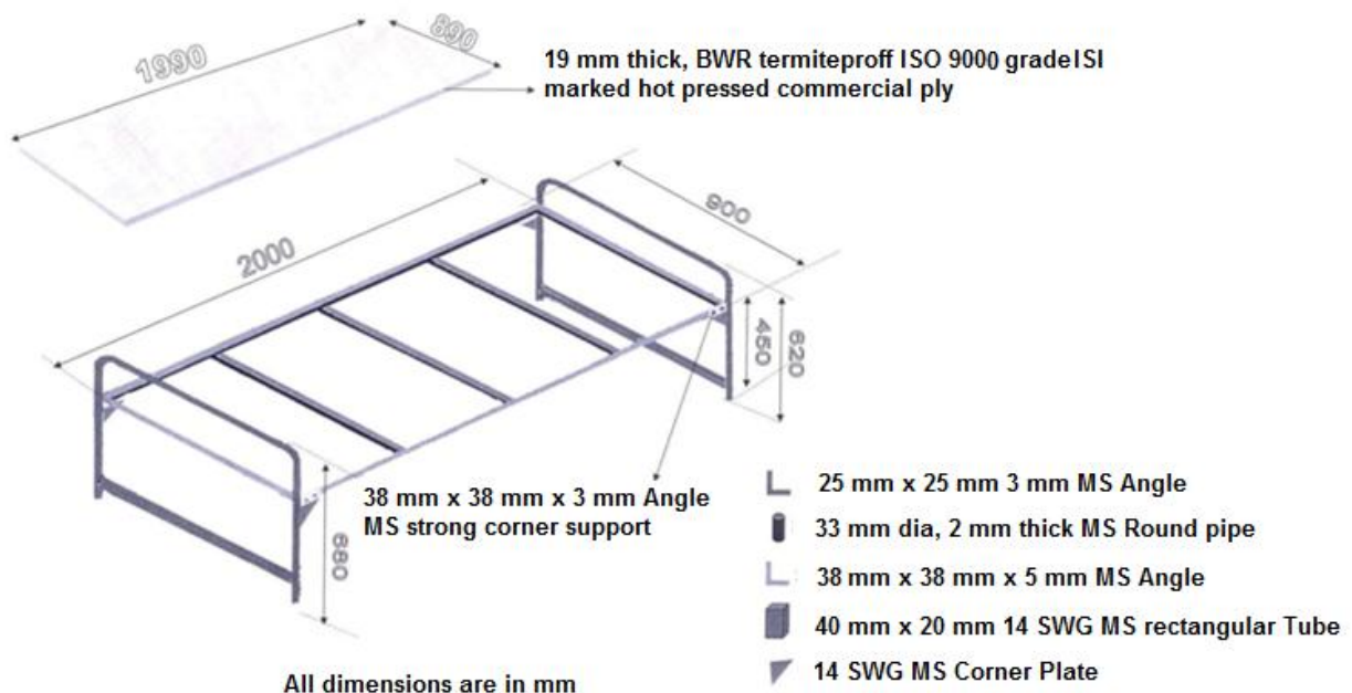
Representative drawing of 'Cots for Hostel Room' (not to scale)
